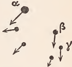
FIG. 12.—OBSERVED PROPER MOTIONS OF STARS IN HEAD OF ARIES.
